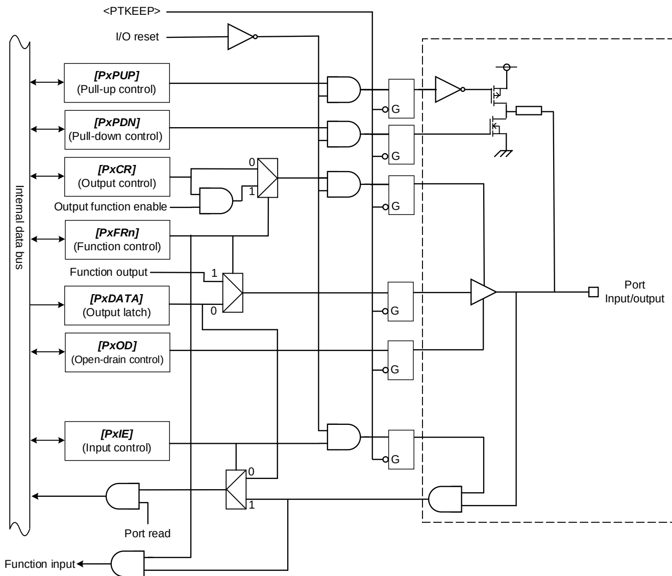
Figure 5.3 Port Type FTU2b
