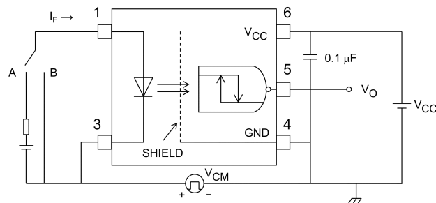
Fig. 12.1.6 Common-Mode Transient Immunity Test Circuit and Waveform
