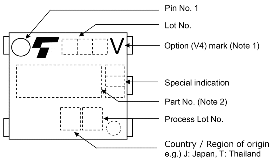
Fig. 16.4 Marking Example
