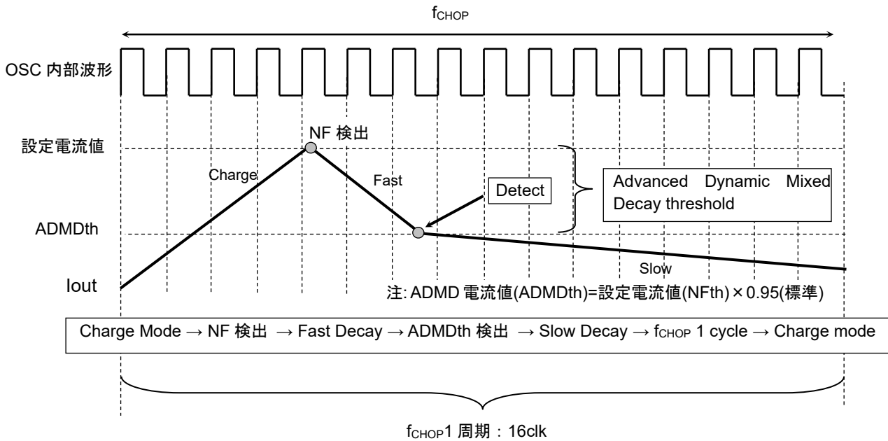
図 6.15 ADMD(Advanced Dynamic Mixed Decay)定電流制御
