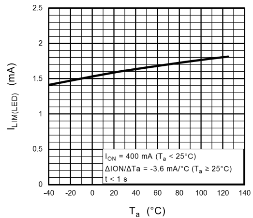
Fig. 12.6 I_{LIM(LED)} - T_a
