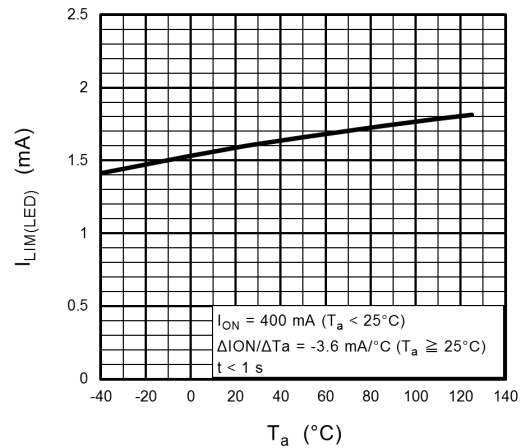
図 12.6 I_{LIM(LED)} - T_a
