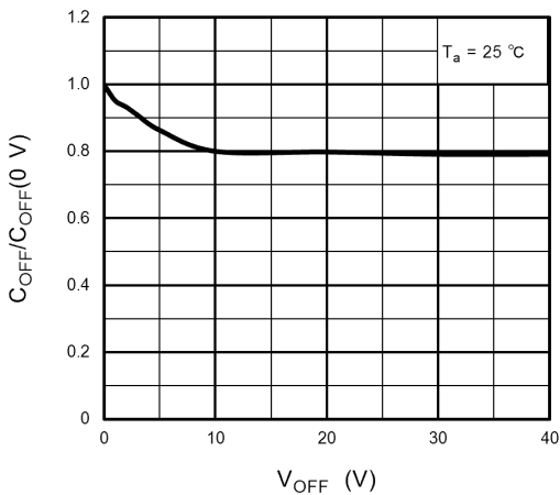
Fig. 12.1.11 C_{OFF}/C_{OFF(0V)} - V_{OFF}
