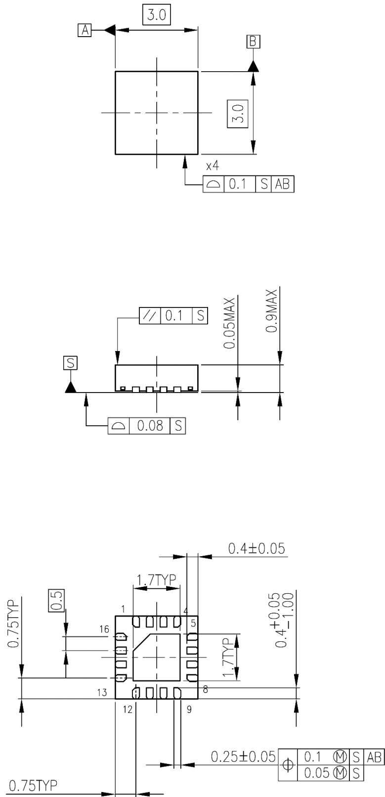
Figure 22 Package Dimensions
