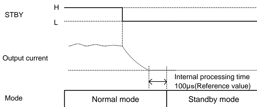
Figure 10.2 STANDBY FUNCTION
