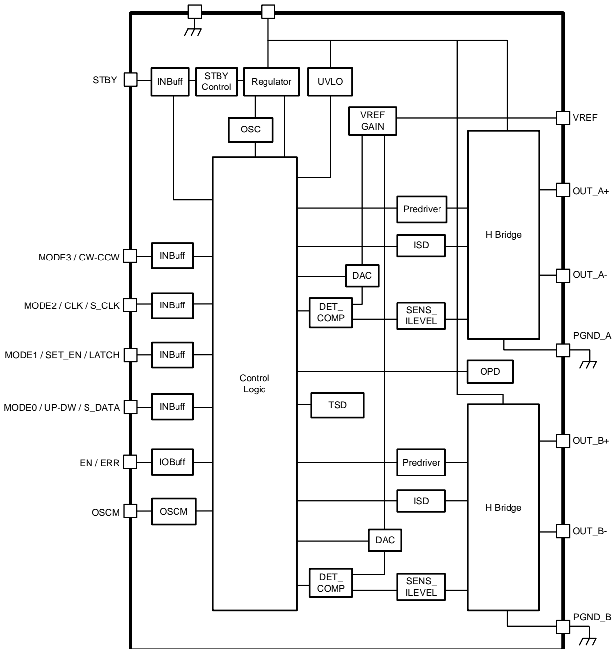
Figure 5 Block diagram
