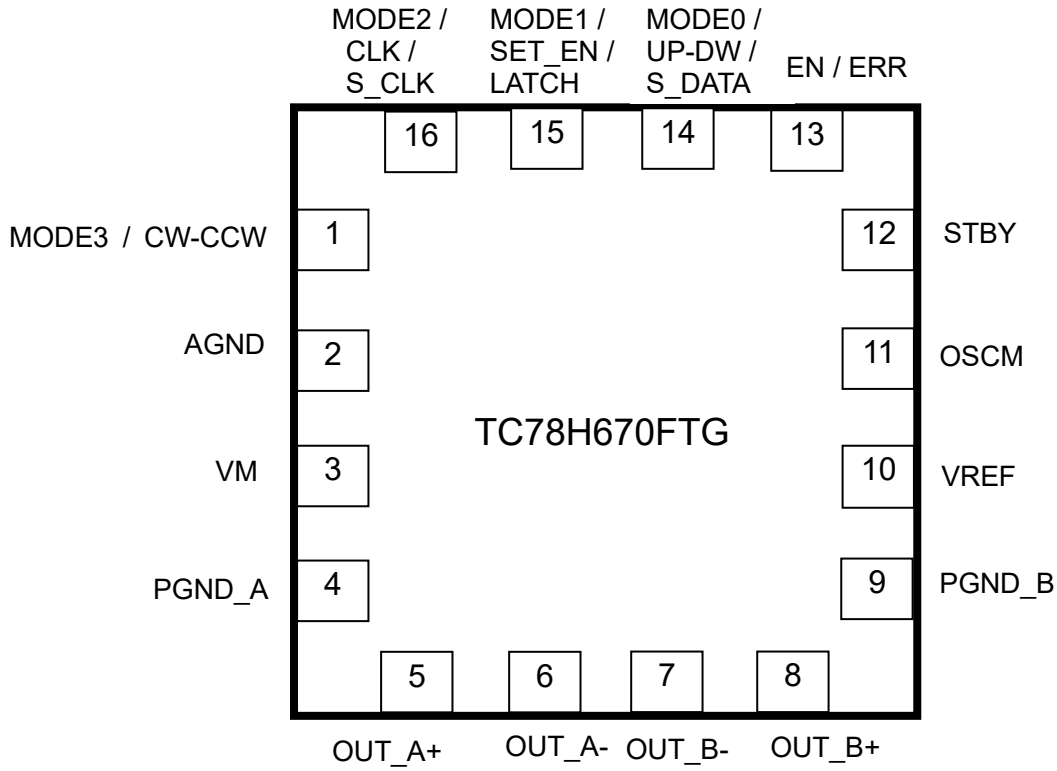
Figure3 Pin Assignment
