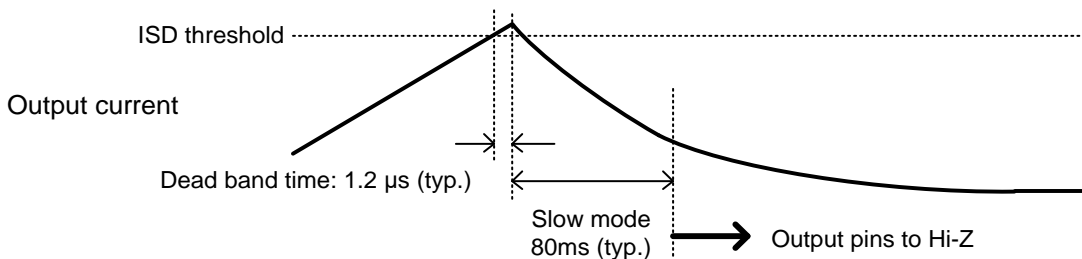
Figure 17 VM-ISD threshold
