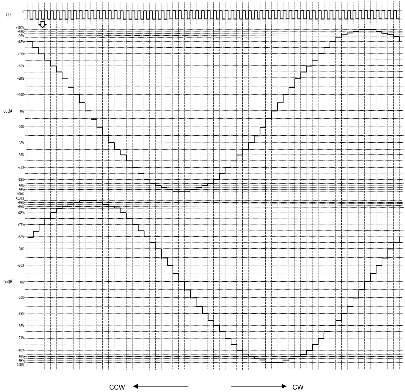
Figure 8.5.5 1/16 step resolution
