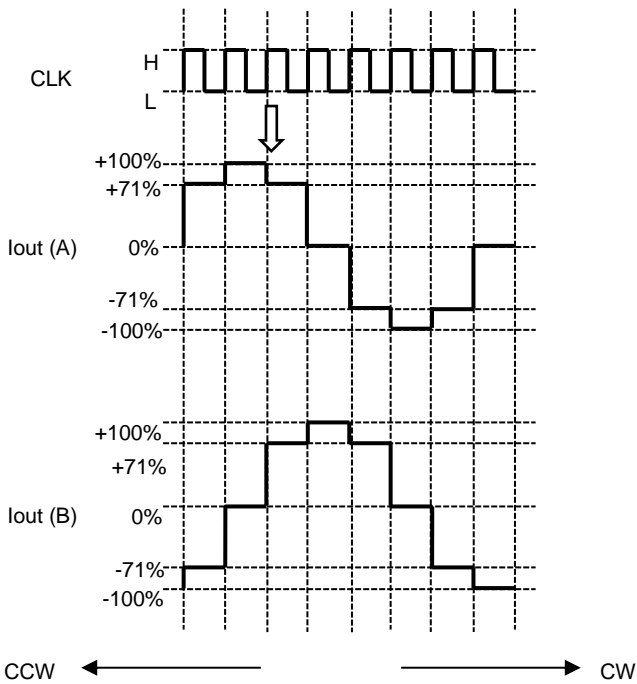
Figure 8.5.2 1/2 step resolution
