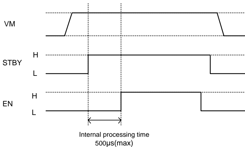
Figure 8.2 ENABLE Function
