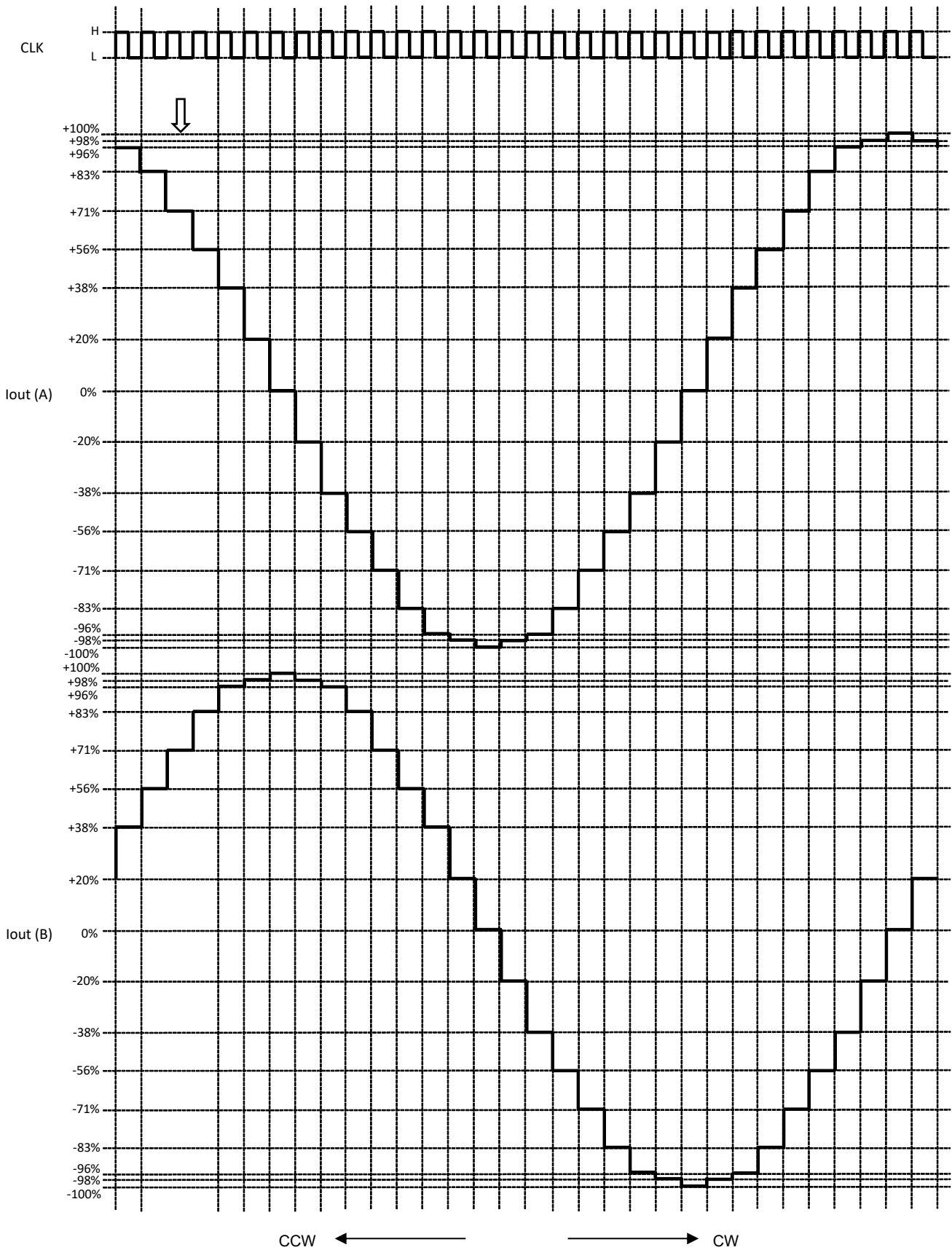
Figure 8.5.4 1/8 step resolution
