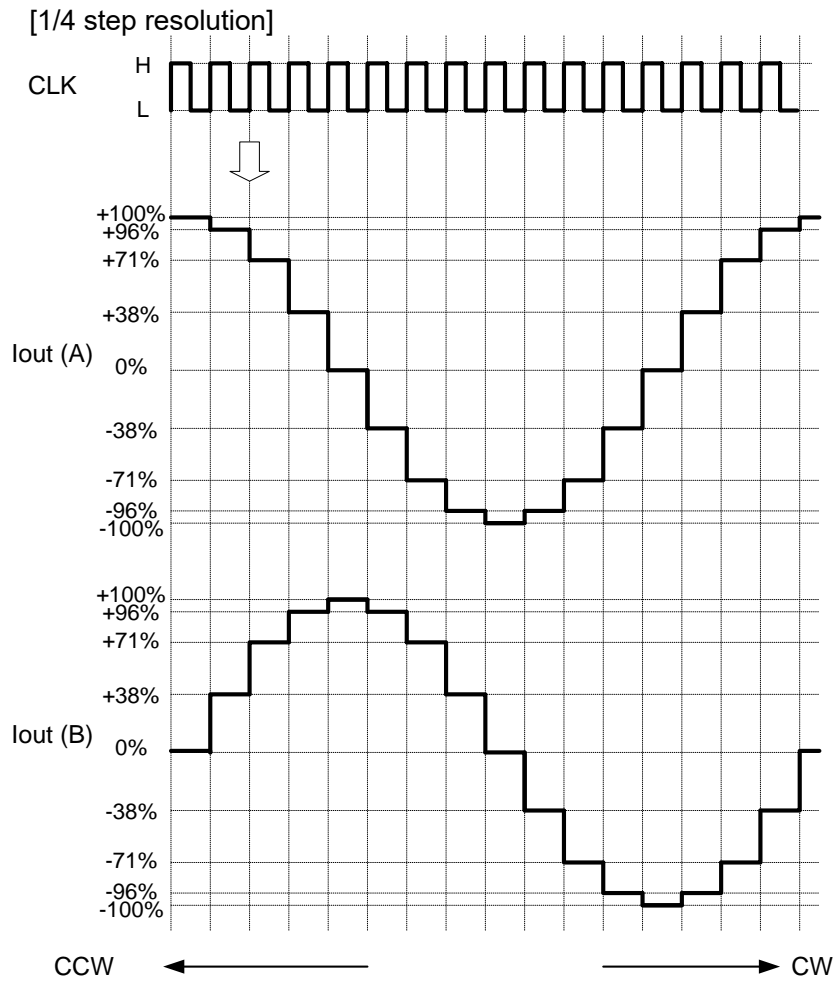
Figure 8.5.3 1/4 step resolution
