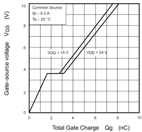
Fig. 8.10 Dynamic Input Characteristics
