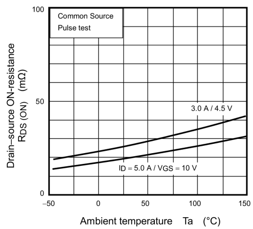
Fig. 8.5 R_{DS(ON)} - T_a
