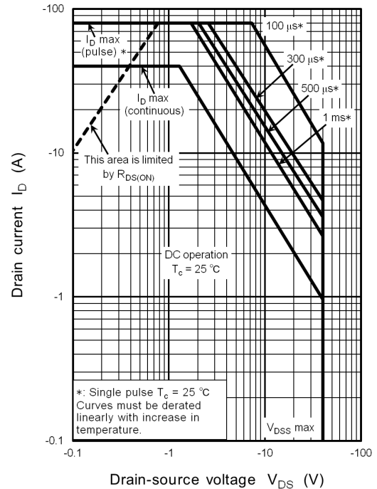
Fig. 8.17 Safe Operating Area (Guaranteed Maximum)
