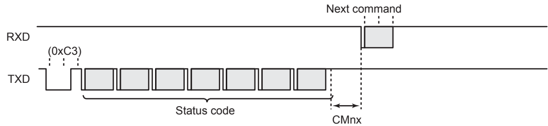
Figure 22-12 Flash Memory Status Output Command
