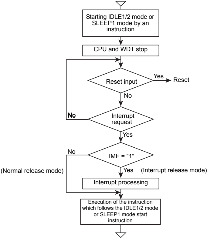
Figure 2-12 IDLE1/2 and SLEEP 1 Modes
