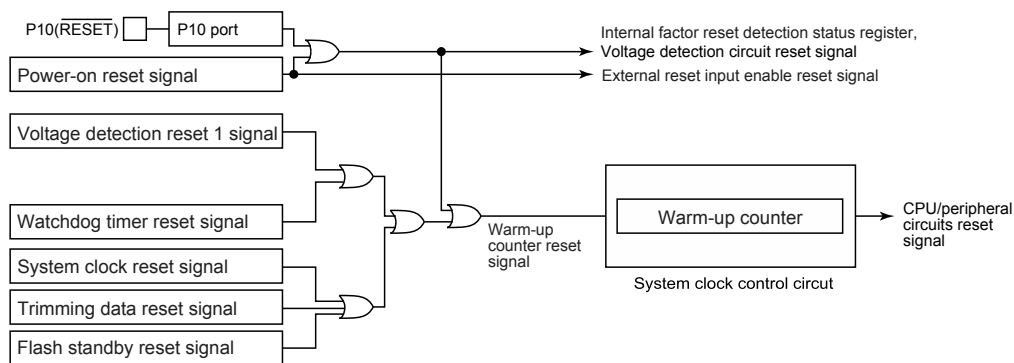
Figure 2-16 Reset Control Circuit
