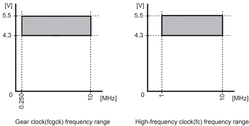
Figure 25-2 Clock gear (fcgck) and High-frequency clock (fc)
