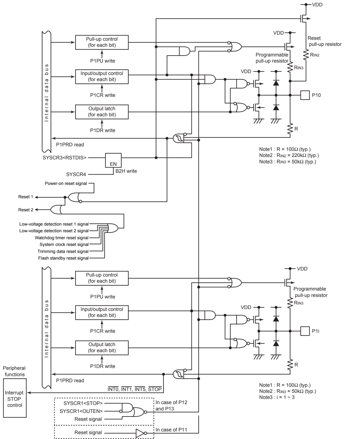
Figure 8-4 Port P1
