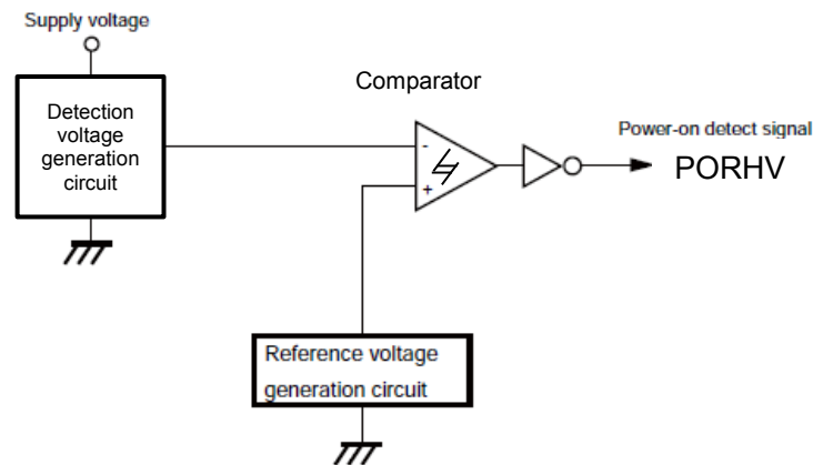
Figure 2.8 Power On Reset Circuit
