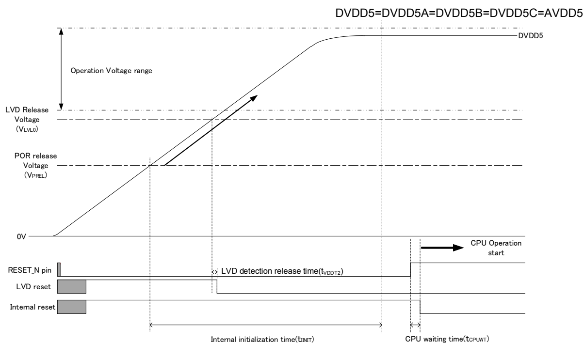
Figure 2.2 Reset operation by a RESET_N pin (1)
