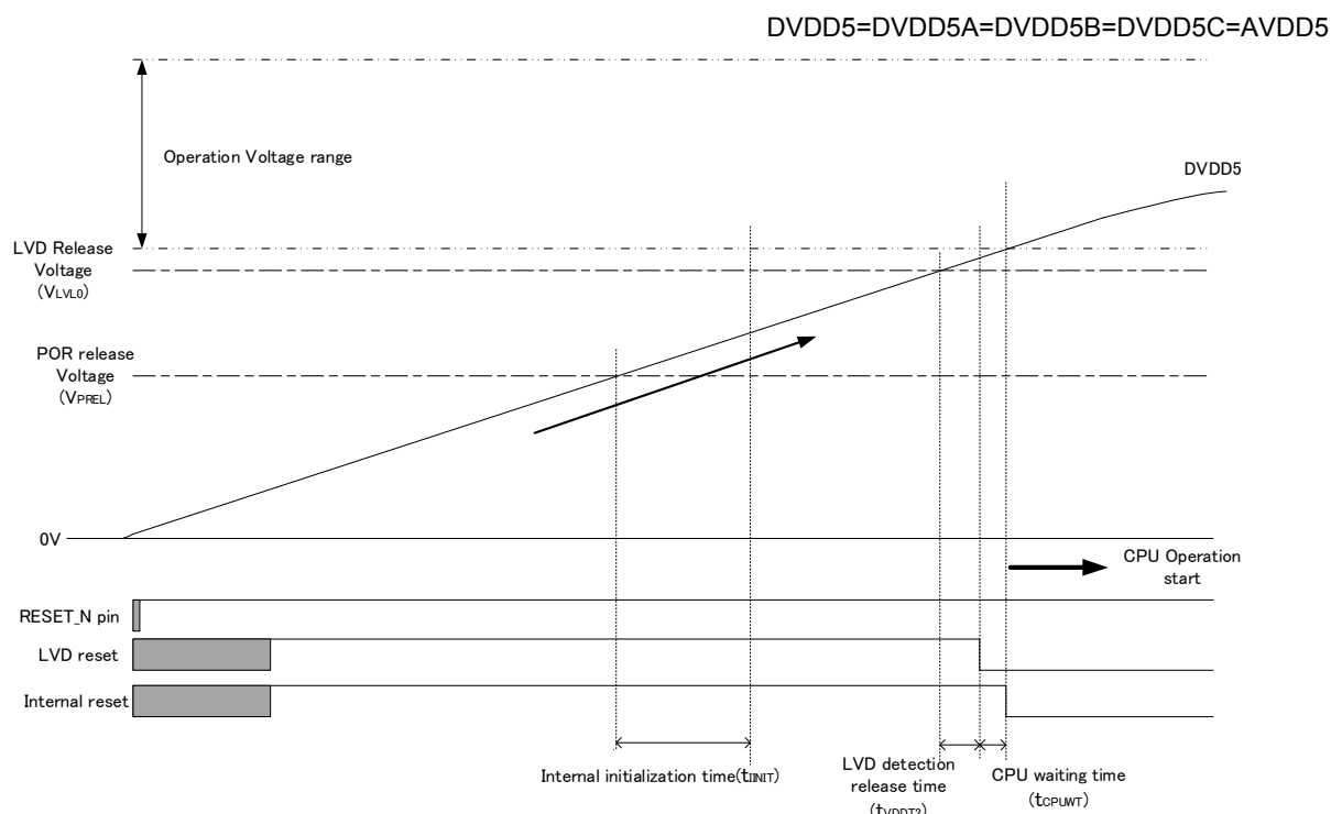
Figure 2.4 The reset operation by LVD reset
