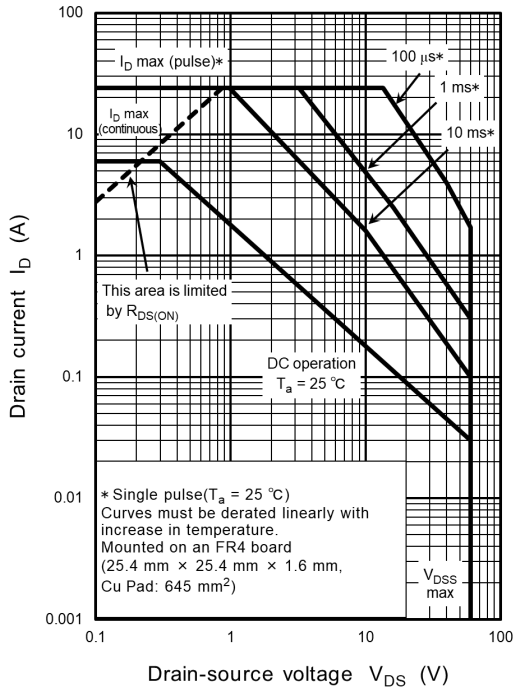
Fig. 9.11 Safe Operating Area
