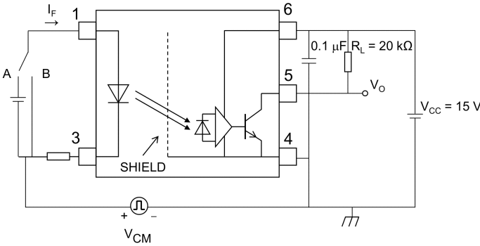
Fig. 12.1.7 Common-Mode Transient Immunity Test Circuit and Waveform
