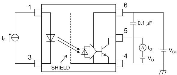
Fig. 12.1.5 I_O Test Circuit
