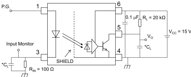
Fig. 12.1.6 Switching Time Test Circuit and Waveform
