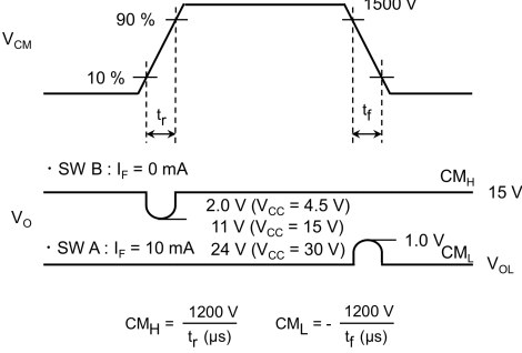
Fig. 12.1.7 Common-Mode Transient Immunity Test Circuit and Waveform
