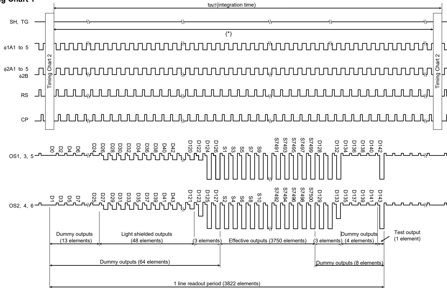
Timing Chart 1
