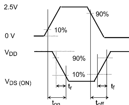
Fig. 7.3.2 Input Waveform/Output Waveform
