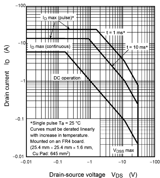
Fig. 9.15 Safe Operating Area
