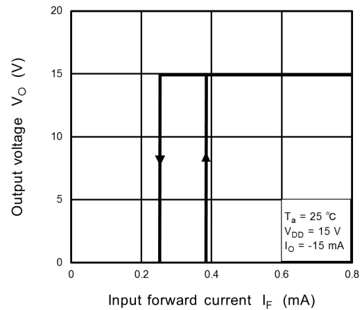
Fig. 12.2.4 V_O - I_F(IHYS)
