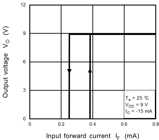
Fig. 12.2.3 V_O - I_F(IHYS)
