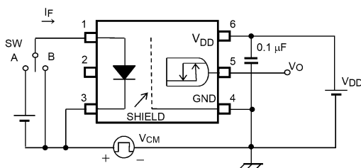
Fig. 12.1.8 Common-Mode Transient Immunity Test Circuit and Waveform
