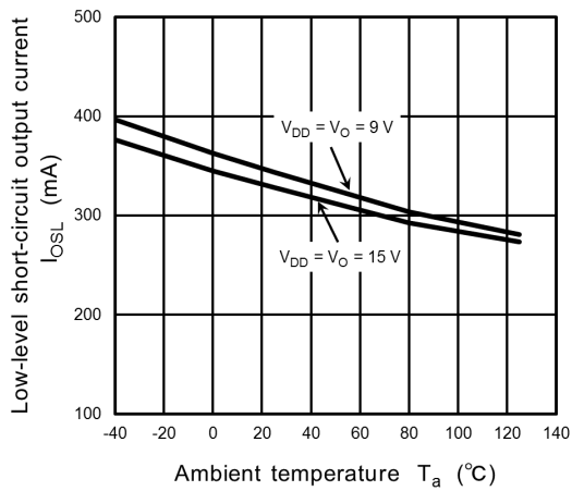
Fig. 12.2.9 I_{OL} - T_a
