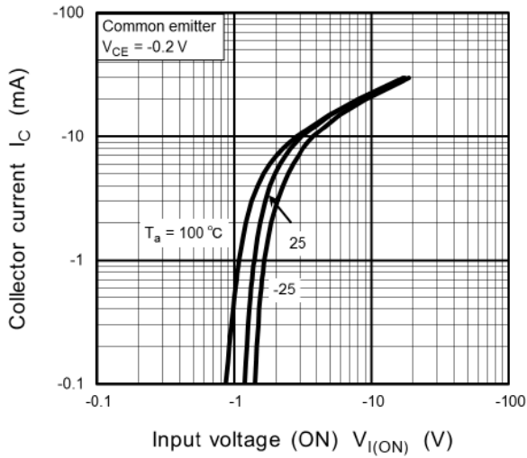
Fig. 11.3 RN2103MFV I_C - V_{I(ON)}
