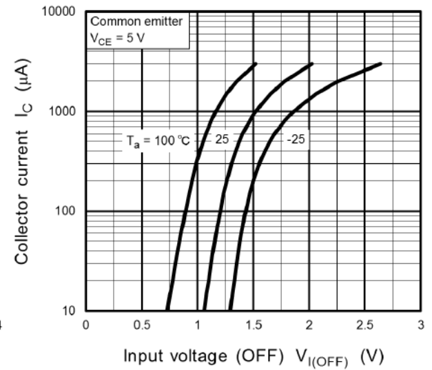
Fig. 11.10 RN1104MFV I_C - V_{I(OFF)}
