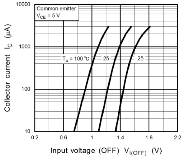
Fig. 11.8 RN1102MFV I_C - V_{I(OFF)}
