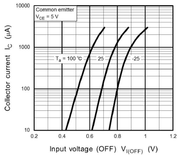
Fig. 11.12 RN1106MFV I_C - V_{I(OFF)}
