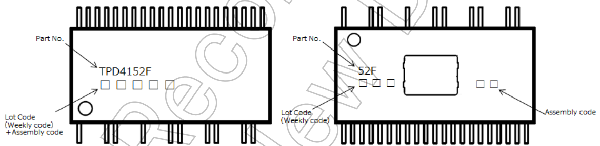
TPD4152F,BF(S)
