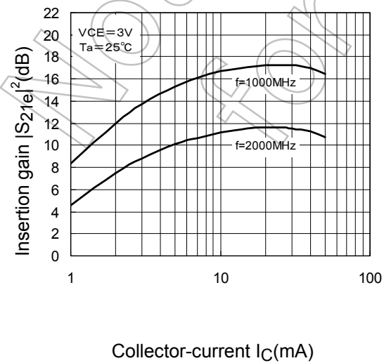
|S_{21e}|^2-I_C
