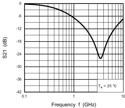
図 8.5 S_{21} - f
