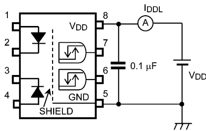
Fig. 12.1.3 I_{DDL} Test Circuit
