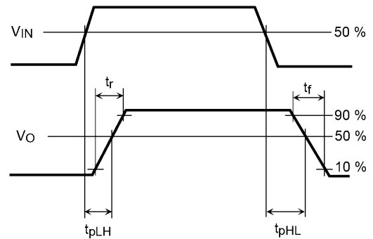
Fig. 12.1.5 Switching Time Test Circuit and Waveform
