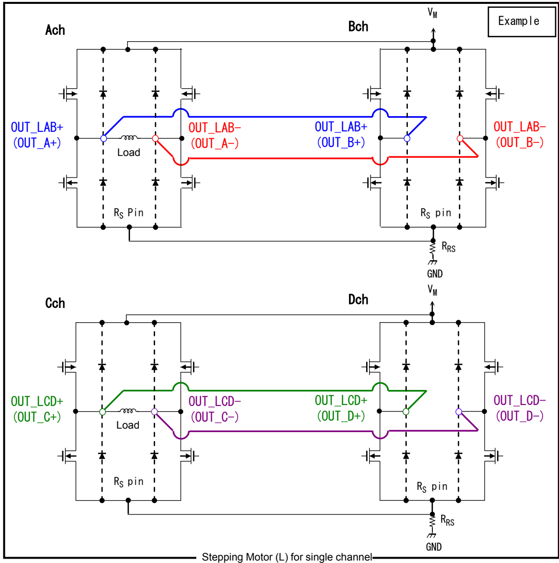
Stepping Motor (L) for single channel
