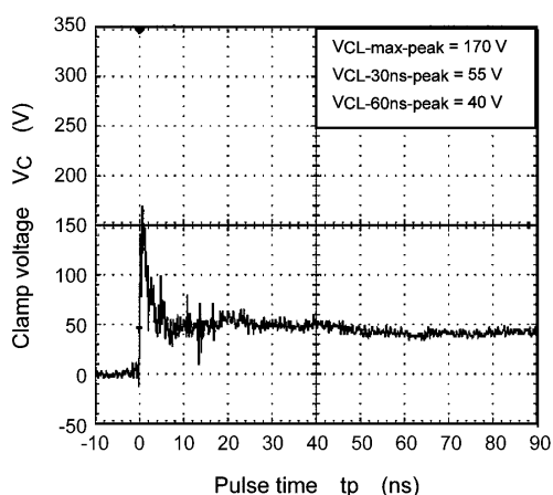
Fig. 9.3 +15 kV (IEC61000-4-2)
