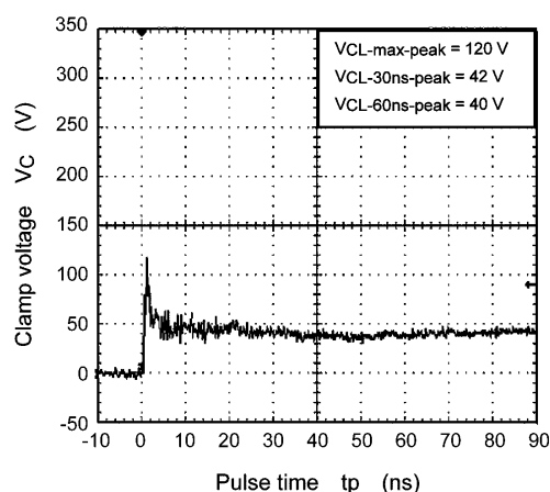
Fig. 9.1 +8 kV (IEC61000-4-2)
