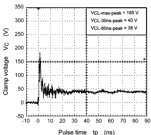
Fig. 10.3 +15 kV (ISO10605)
