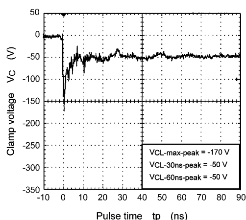
Fig. 9.2 -8 kV (IEC61000-4-2)
