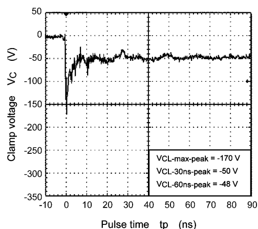
Fig. 10.2 -8 kV (ISO10605)
