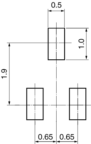
Fig. 6.1 Land Pattern Dimensions (Unit: mm)
