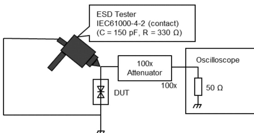
Fig. 9.5 IEC61000-4-2 (Contact)
