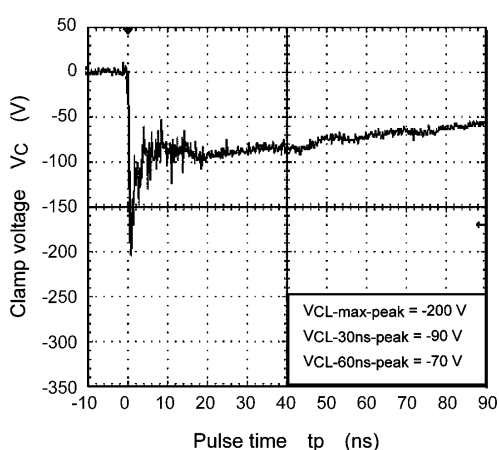
Fig. 9.4 -15 kV (IEC61000-4-2)
