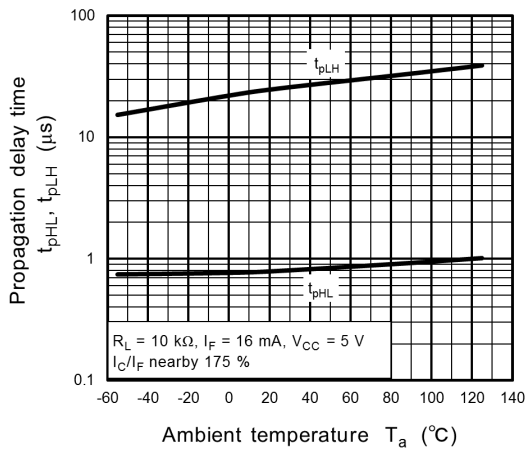
Fig. 11.17 t_{pHL}, t_{pLH} - T_a
