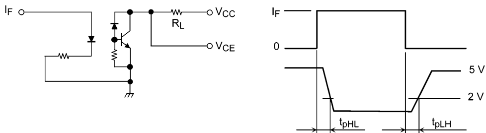
Fig. 10.1 Switching Time Test Circuit and Waveform
