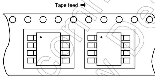
Figure 1 Device Orientation
