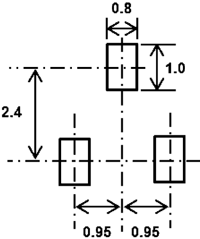
Fig. 7.1 S-Mini (Unit: mm)
