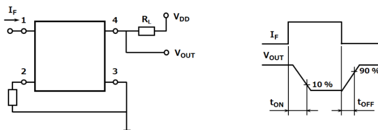
Figure 11.1 Switching Time Test Circuit and Waveform
