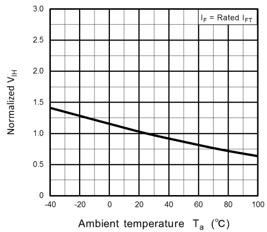
Fig. 12.12 Normalized V_{HH} - T_a
