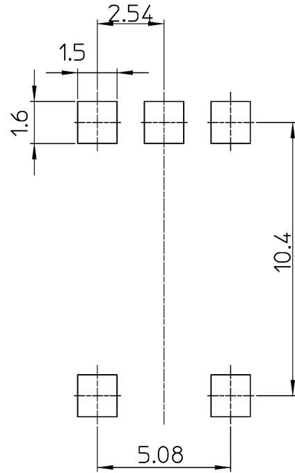
Fig. 14.2 TLP3062AF Lead forming and taping option (LF4), (TP4)
