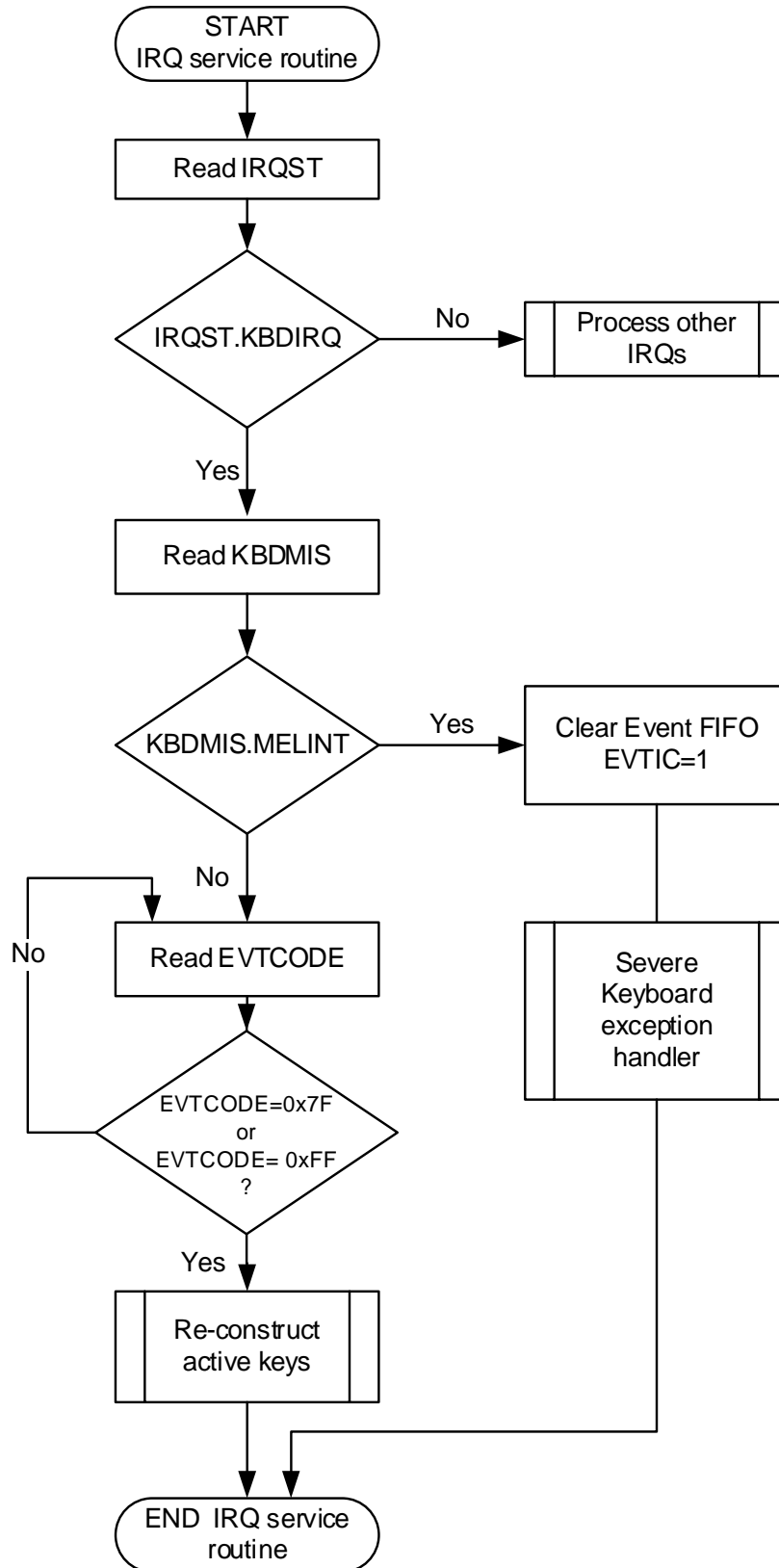
Figure 10.7 Interrupt handler for Event FIFO
