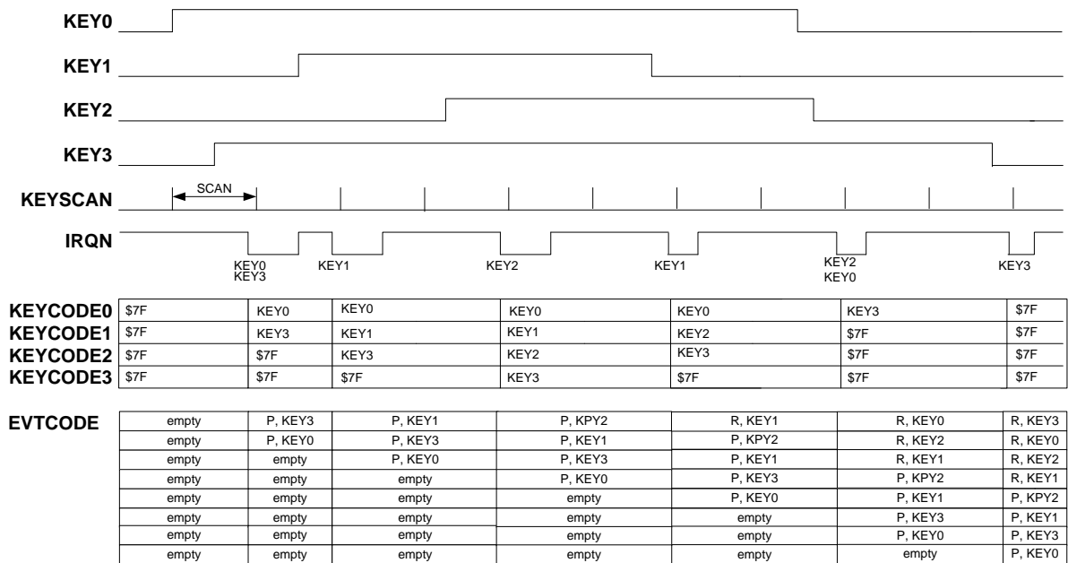
Figure 10.5 Multiple Key-press
