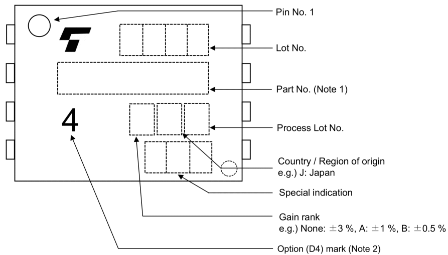
Fig. 16.4 Marking Example
