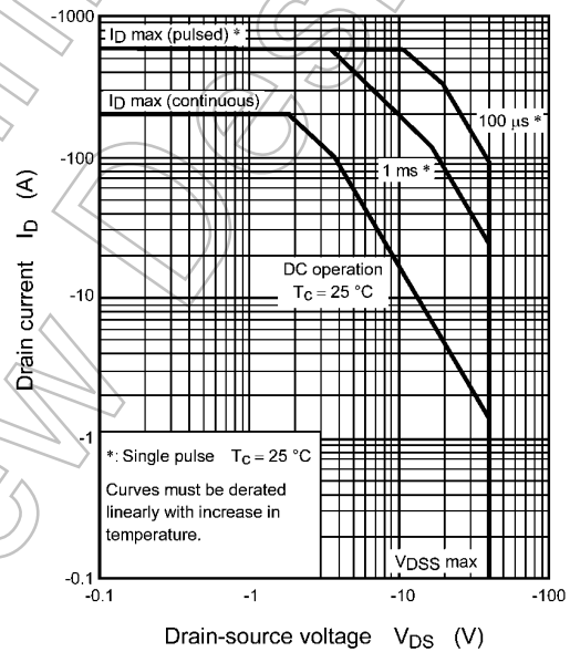
Fig. 9.13 Safe Operating Area (Guaranteed Maximum)
