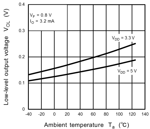
Fig. 13.2.4 V_{OL} - T_a
