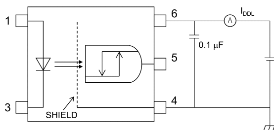
Fig. 12.1.3 I_{DDL} Test Circuit
