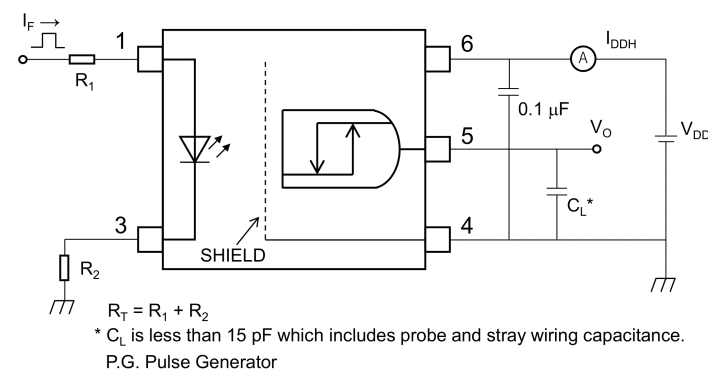
Fig. 12.1.5 Switching Time Test Circuit and Waveform
