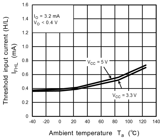
Fig. 13.2.9 I_{FHL} - T_a
