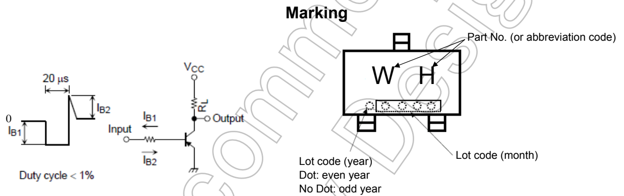
Figure 1. Switching Time Test Circuit
