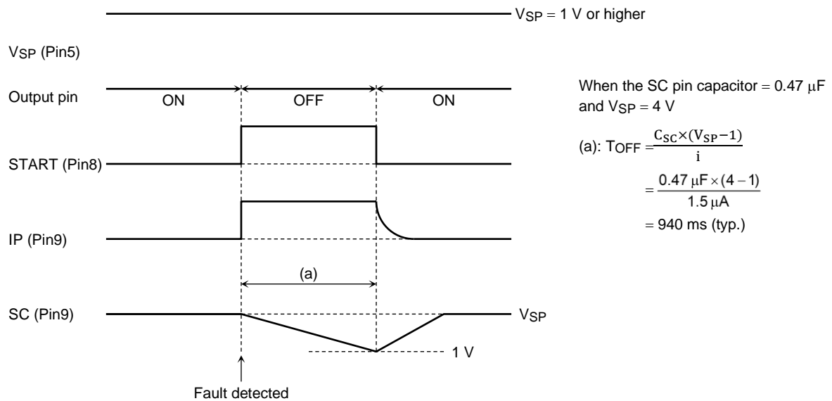
Figure 6.7 Fault protection
