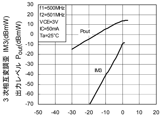
IM3/P out -P in
