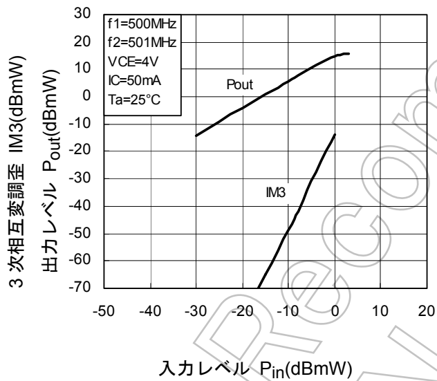
IM3/P out -P in
