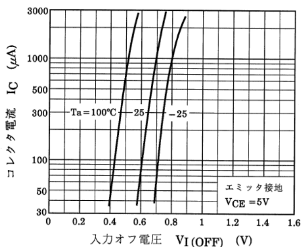
図 9.4 RN1911FE I_C - V_{I(OFF)}
