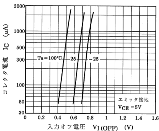
図 9.3 RN1910FE I_C - V_{I(OFF)}
