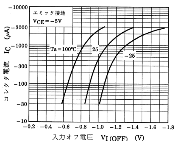
図 13.4 Q2 I_C - V_{I(OFF)}
