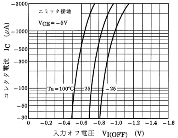
図 10.4 RN2907 I_C - V_{I(OFF)}
