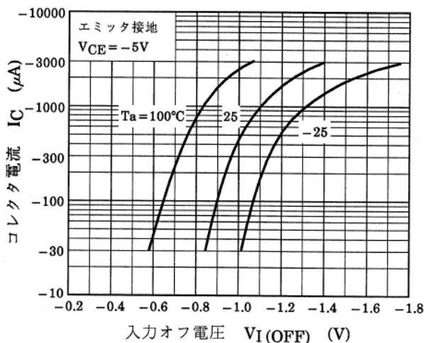
図 10.5 RN2908 I_C - V_{I(OFF)}
