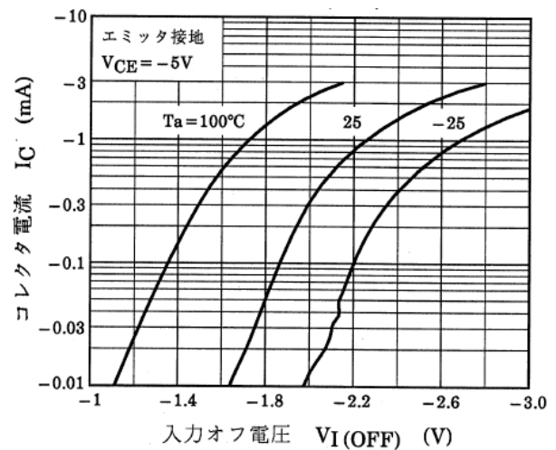
図 10.6 RN2909 I_C - V_{I(OFF)}
