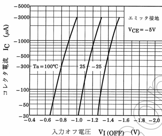
図 9.9 RN2423 I_C - V_{I(OFF)}
