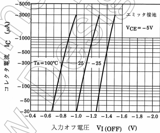
図 9.4 RN2422 I_C - V_{I(OFF)}
