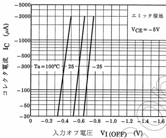
図 9.15 RN2425 I_C-V_{I(OFF)}
