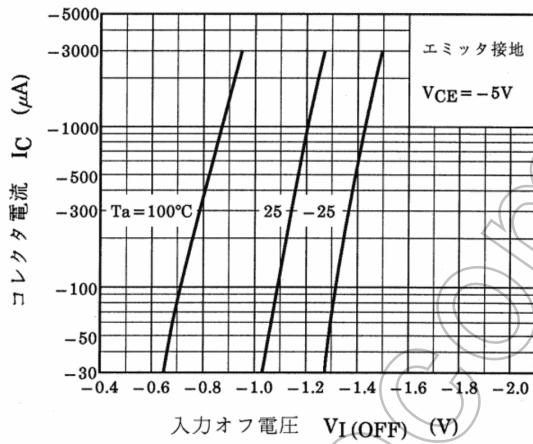
図 9.3 RN2421 I_C - V_{I(OFF)}
