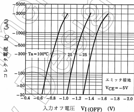
図 9.10 RN2424 I_C - V_{I(OFF)}
