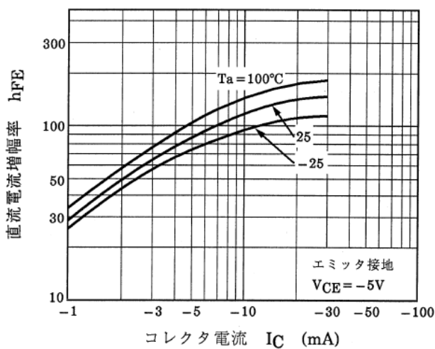
図 10.9 RN2109 h_{FE}-I_C
