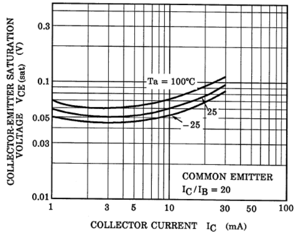
Fig. 10.22 RN1904 V_{CE(sat)}-I_C
