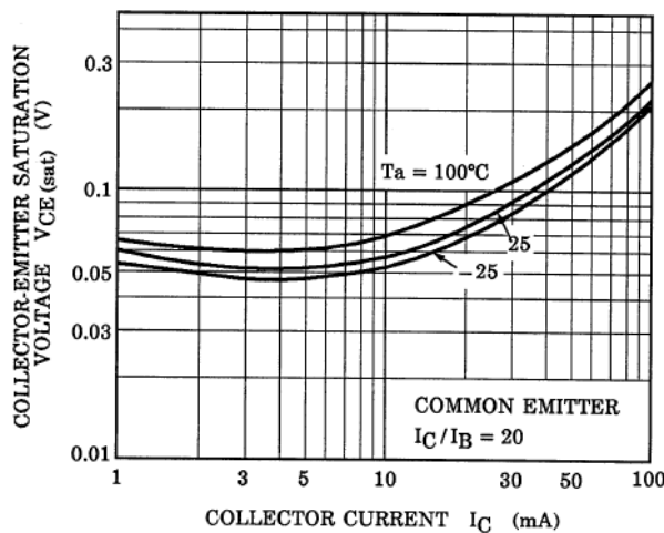
Fig. 10.23 RN1905 V_{CE(sat)}-I_C
