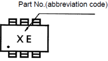
Fig. 9.5 Marking RN1905
