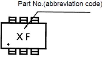
Fig. 9.6 Marking RN1906
