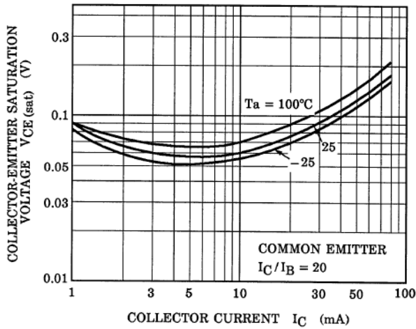
Fig. 10.21 RN1903 V_{CE(sat)}-I_C
