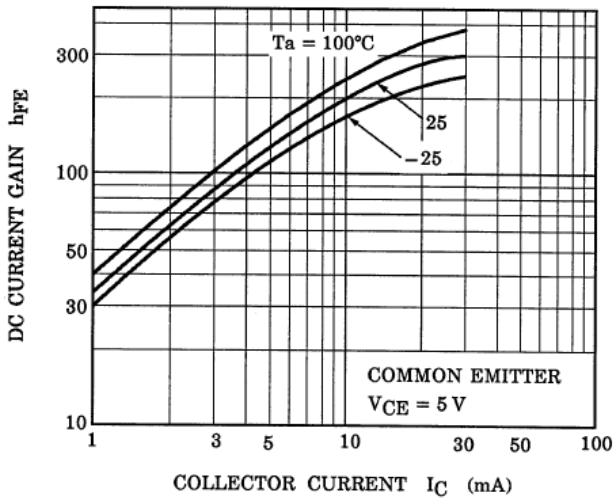
Fig. 10.9 RN1409 h_{FE}-I_C
