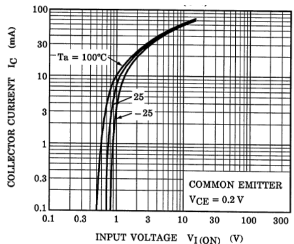
Fig. 10.6 RN1406 I C -V I(ON)
