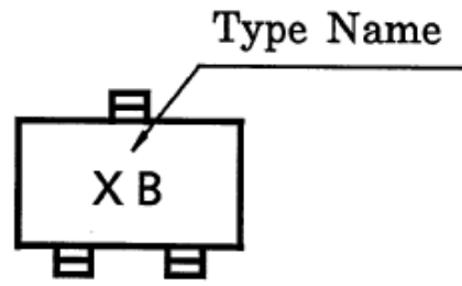
Fig. 9.2 Marking RN1402
