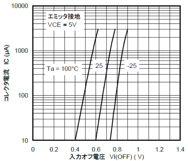
図 10.6 RN1314 I_C - V_{I(OFF)}
