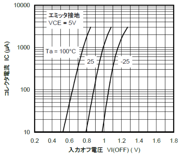
図 10.8 RN1316 I_C - V_{I(OFF)}
