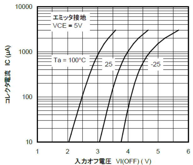
図 10.10 RN1318 I_C - V_{I(OFF)}
