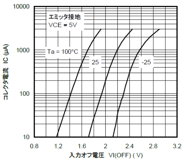
図 10.9 RN1317 I_C - V_{I(OFF)}
