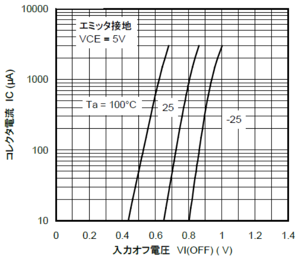
図 10.7 RN1315 I_C - V_{I(OFF)}
