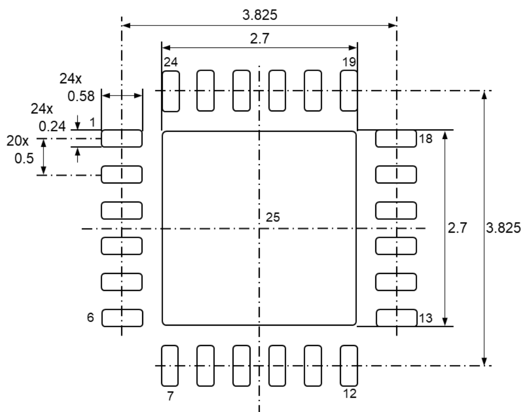
Figure 13.2 Land Pattern Dimensions for Reference only
