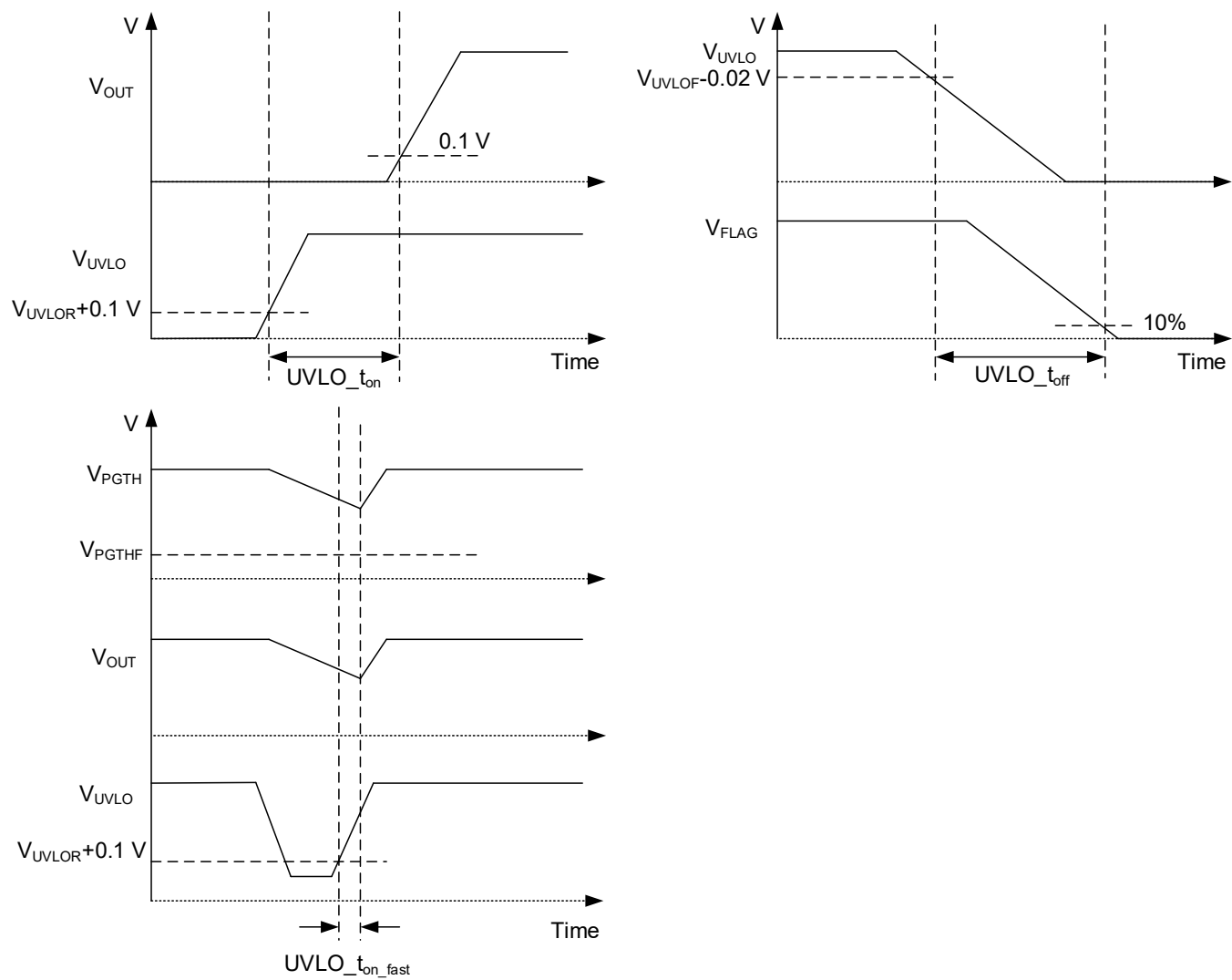
Figure 11.1 UVLO characteristics
