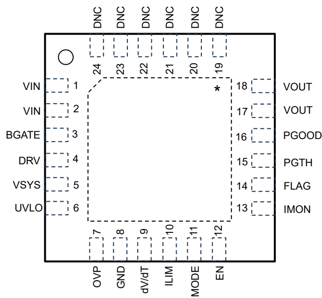
Figure 5.1 Pin Assignments
